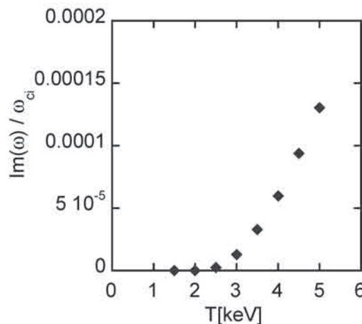
Fig.2 The growth rate of the 2 nd harmonic waves are plotted as a function of ion temperature
