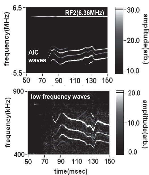
Fig.1 Frequency spectra of AIC-modes (upper figure) and low frequency waves which have differential frequencies between the heating wave (6.36 MHz) and the AIC-modes (lower figure).
