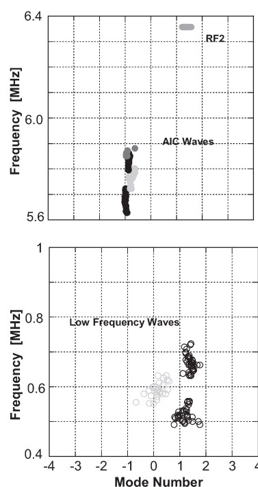
Fig.2 Azimuthal mode structures of the heating wave, the AIC modes (upper) and the LF waves (lower).
