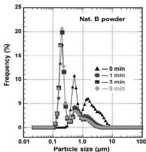
Fig.1 Typical particle size distributions of the boron powder after various vibrated milling time
