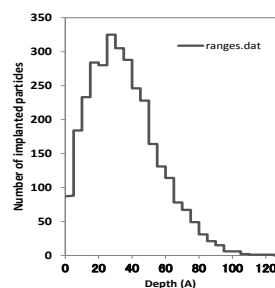
Fig. 1 Implantation profile of H in Fe at E=100\text{eV} .
