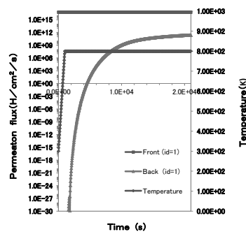
Fig. 2 Plasma-driven permeation flux at 800K.
