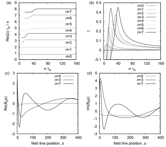
Fig. 1: Eigenfrequency \Omega and eigenfunction B_0 \psi of shear Alfvén modes obtained by equation (3) with the impedance ratio \alpha = 5 and the ionospheric cavity of v_A . Panels (a) and (b) show real and imaginary parts of \Omega , normalized by the Alfvén transit time \tau_A as a function of the ionospheric electric drift frequency \sigma , for lower eight harmonics n = 0-7 ; \gamma = \text{Im}(\Omega)\tau_A/\pi . Field-line distribution of (c) real and (d) imaginary parts of B_0 \psi for the maximum \gamma of harmonics n = 0, 3 , and 7 .
