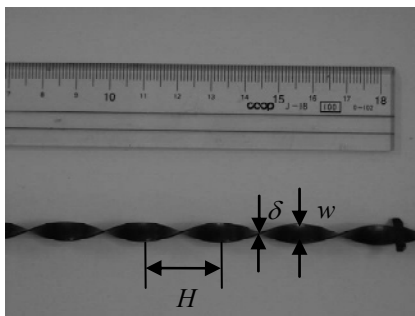
Fig. 1 Photograph of SUS304 twisted tape coated with epoxy resin.
