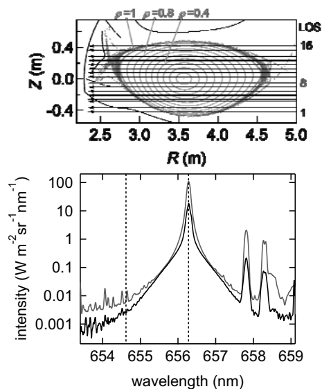
Fig.2. (a) A poloidal cross section of LHD and LOSs for the emission observation. (b) The observed Balmer- \alpha spectra for LOS1 (black curve) and LOS8 (gray curve).
