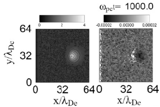
Fig. 2: Electron density distribution (the left panel) and distribution of the y component of electric current density (the right panel) in the x - y plane at z = L_z/2 at \omega_{pe}t = 1000 .
