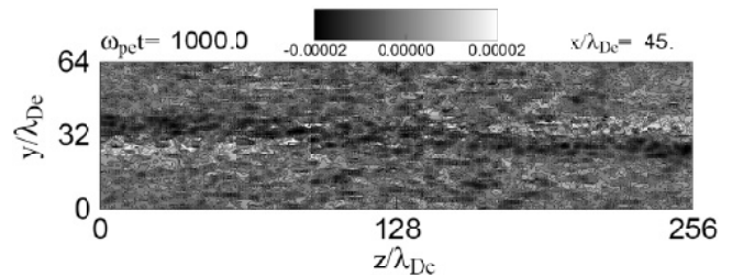
Fig. 3: Distribution of the z component of electric current density in the z - y plane at x = 45\lambda_{De} at \omega_{pe}t = 1000 .
