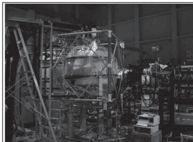
Fig. 2 The photograph of the CPD during vacuum leak check at the experimental hall of TRIAM-1M.
