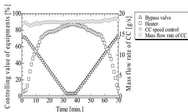
Fig. 1. Time trend of the heater power while changing the opening degree of the bypass valve at a constant rate under the constant rotational speed of the cold compressors with the automatic flow control of the cold compressors to be 18 g/s by the heater.
