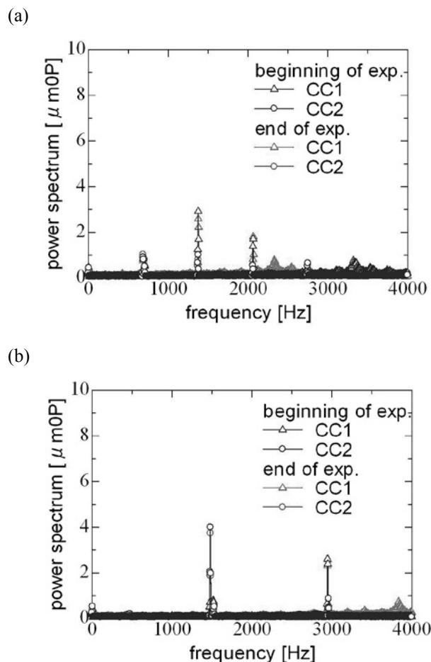
Fig. 2. Power spectrum of the rotational vibrations by FFT analysis of the displacement of the rotor shafts before and after the 16 th LHD experiment campaign; (a) power spectrum in the waiting operation, (b) power spectrum in the rated operation.
