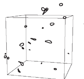
FIG. 2: Distribution of the vortex rings at T = 1.6K
