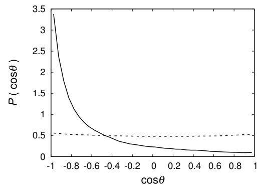
Fig. 1: The PDF of the cosine of the angle \theta between segments of vortex axes at the length scale \ell_c \approx 40\eta . Solid line, the PDF conditioned by the distance r between the axes as 0.8 < r/\ell_c < 0.9 ; dashed line, 3.0 < r/\ell_c < 3.5 .
