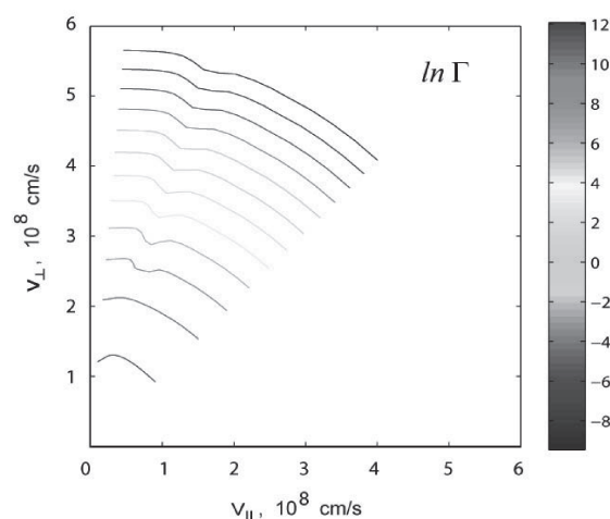
Fig. 2. Energy and angle-resolved flux of H^0 particles.
