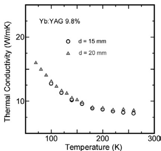
Fig. 2. Experimental results of thermal conductivity for 9.8% doped Yb:YAG ceramics.
