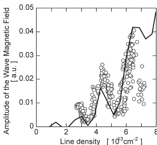
Fig.1 The amplitude of the wave field, measured with a magnetic probe, as a function of the line density. A solid line indicates the calculated amplitude in the GAMMA 10 configuration.
