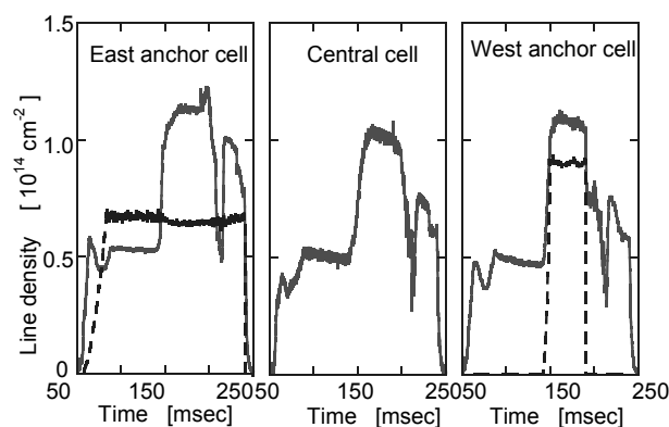
Fig.2 Temporal evolution of the line density in the east anchor, central and west anchor cells when direct ICRF powers are injected in both east and west anchor cells.
