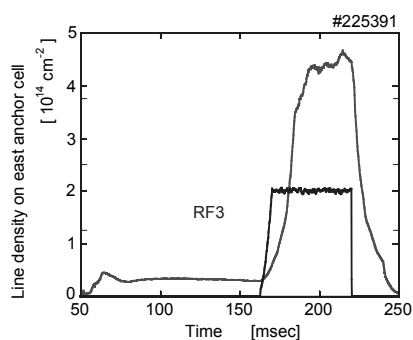
Fig.1 Temporal evolution of the line density in the east anchor cell when direct ICRF power (RF3) is injected in the anchor cell.
