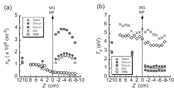
Fig. 2. Axial distributions of plasma parameters: Electron density n_e (a) and electron temperature T_e (b) for three different mesh grids and two different MF fields. The end plate is set at z_{\text{end}} = -10.5 cm. Experimental conditions: P_{\text{rf}} = 200 W, p(H_2) = 3 mTorr, and grid biasing voltage V_g = -50 V.
