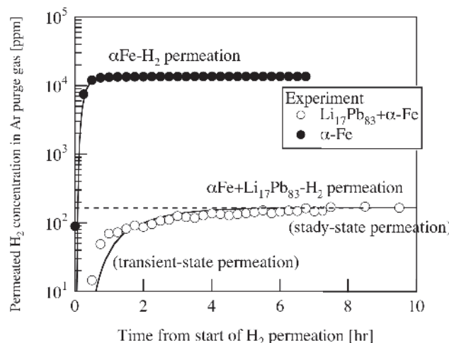
Fig. 2 Comparison between experiment and calculation for transient hydrogen permeation behavior in \text{LiPb}^3
