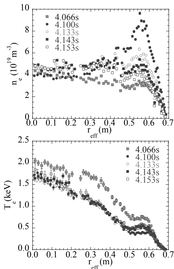
Fig. 1: profiles of (a)electron density and (b)electron temperature in after the injection of an Hydrogen pellet.
