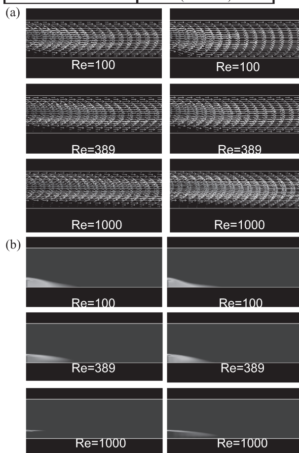
Figure 2 Two-dimensional velocity vector and temperature contour at Pr = 7.1 : (a) velocity vector, left hand side is non-MHD, right hand side is MHD, (b) temperature contour, left hand side is non-MHD, right hand side is MHD
