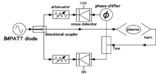
Fig. 1: Schematic of the developed interferometer system.
