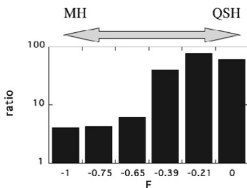
Fig. 1: Ratio of the amplitude of the dominant to secondary mode is plotted as a function of field reversal parameter F of initial RFP configuration.
