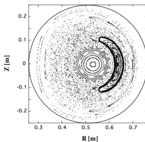
Fig. 2: Poincare plot of magnetic field lines from ORBIT code with experimental data in RELAX QSH phase. Thick curve indicates a separatrix of a conserved flux surface due to m = 1/n = 5 mode.
