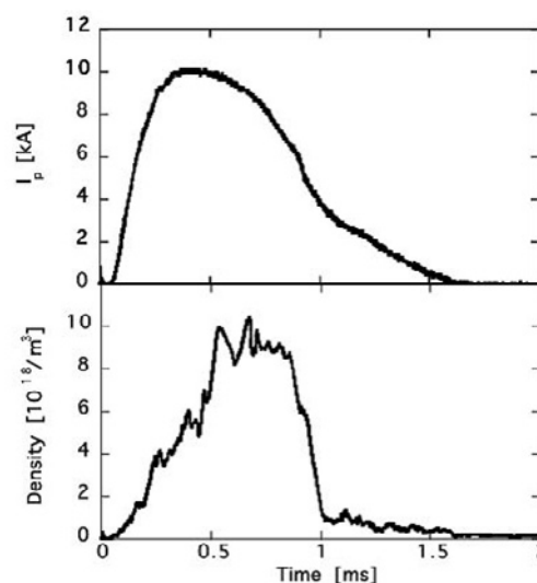
Fig. 2: Time evolution of plasma current and line averaged electron density.
