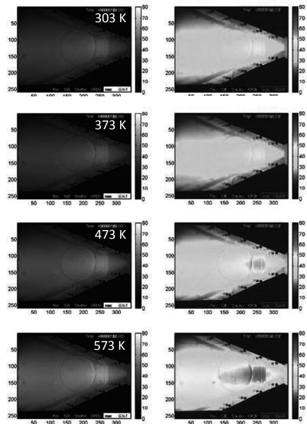
Fig. 2 Evolution of spatial profile of H\alpha line intensity when the target temperature was increased step by step. The target temperatures are indicated in the images. The left column is for raw images and the right column is for false-color images.
