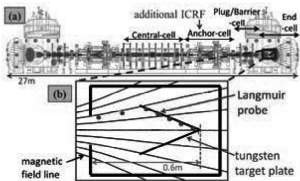
Fig.1 Schematic view of (a) GAMMA 10/PDX and (b) D-module.
