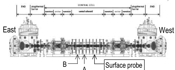
Fig.1 Schematic view of GAMMA 10 and locations of long-term samples (A, B) and a surface probe.
