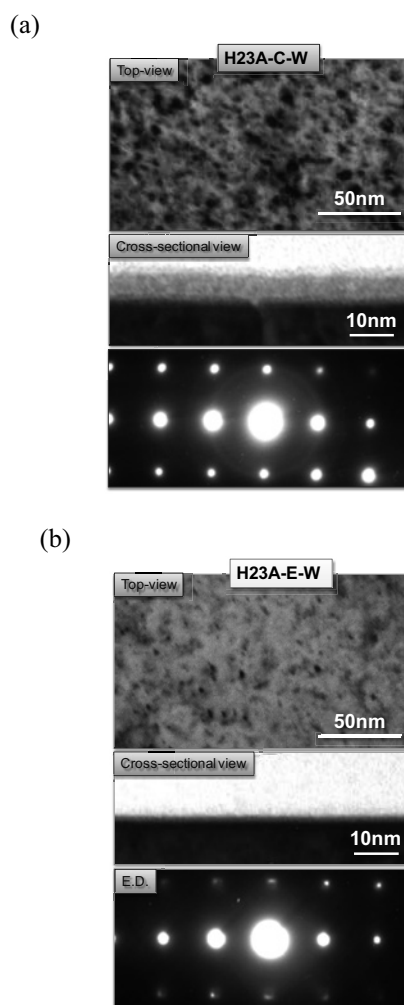
Fig. 3 Top view and cross-sectional view of TEM images, and electron diffraction pattern of (a) the thinned tungsten specimen that was set at the central position and (b) that at the east position.
