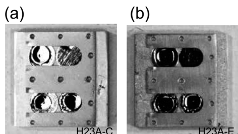
Fig.2 Sample holders with TEM specimens (a) at the central position indicated with "A" in Fig. 1 and (b) at the east position indicated with "B" in Fig. 1.
