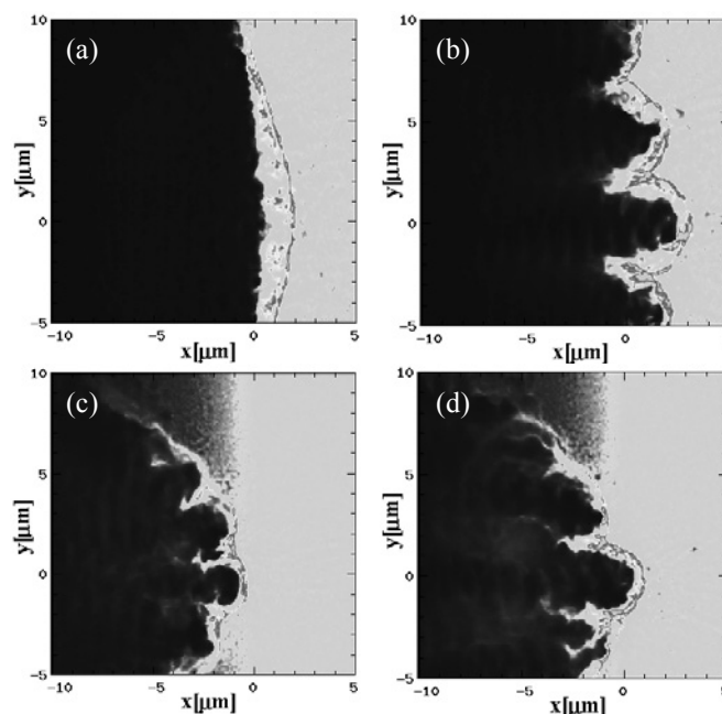
Fig.1. Electron density profiles at 500fs for different pre-plasma scale lengths and the single/double beam.
