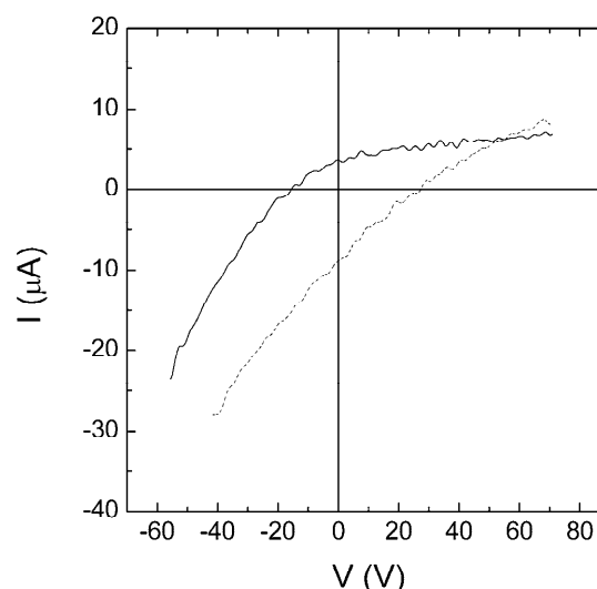
Fig. 2. Example of the obtained V - I curves using the two electrodes, Nos. 1 and 4, as a double probe (solid line) and the curve obtained with reversed polarity (dotted line).
