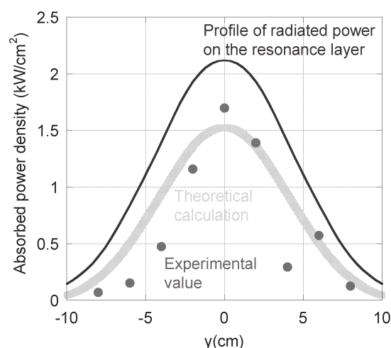
Fig.1 Distribution of the absorbed power density on the resonance layer
