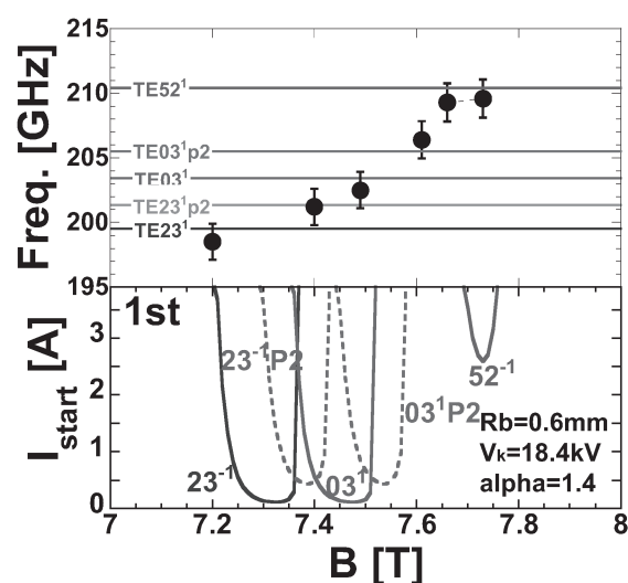
Fig.1 The upper panel plots the measured frequency as a function of the magnetic field strength at the cavity. The horizontal lines labeled by mode number indicate the resonance frequencies of each mode. The lower panel shows the starting current of each mode.
