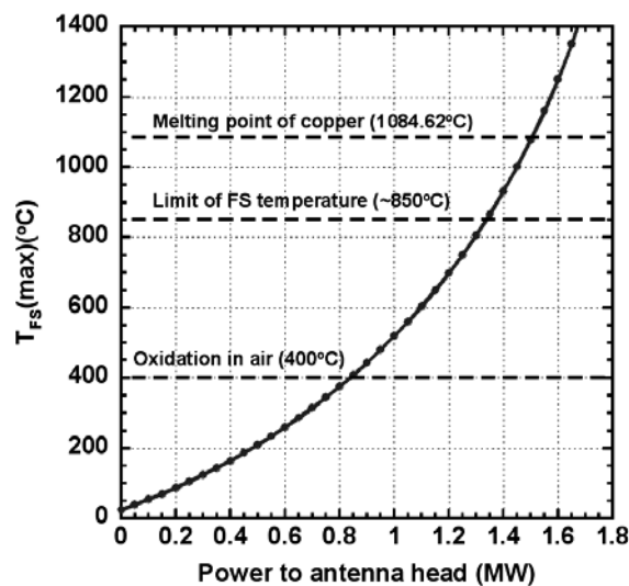
Fig. 3 Estimated temperature on Faraday shield.
