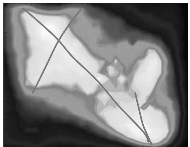
Fig. 3: Bolometric image of radiated power at LHD port 10-O IRVB during island assisted detached plasma in LHD.
