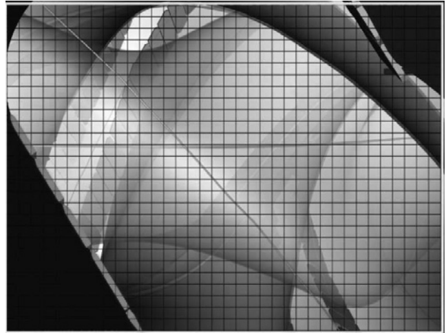
Fig. 1: CAD of FoV of IRVB at port 10-O in LHD.
