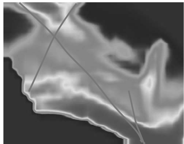
Fig. 2: Synthetic image of radiated power at LHD port 10-O IRVB derived from results of EMC-3 EIRENE code for island assisted detached plasma in LHD.
