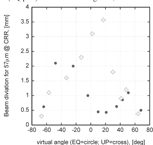
Fig.3. The beam displacement for EQ and UP port 'fun-like' beams, for the 57 \mu\text{m} due to refraction varies from chord to chords.
