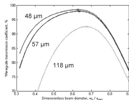
Fig.1. Calculated optimized waveguide diameter of 40 mm for the dielectric waveguides for 48, 57 and 118 \mu\text{m} .
