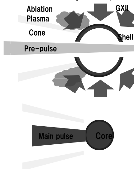
Fig. 1. Hole-cone-hole-shell target.
