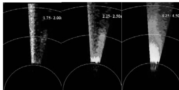
Fig.1. The pitch angle distribution with plasma (left) B=-0.43\text{T} , (center) B=-1.2\text{T} , (right) V=-2.7\text{T} .
