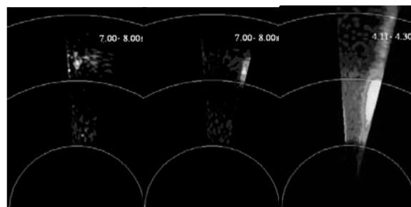
Fig.2. The pitch angle distribution without plasma (left) B=-0.43\text{T} , (center) B=-1.2\text{T} , (right) V=-2.7\text{T} .
