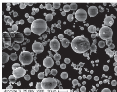
Fig. 1 Photograph of a Ti dust mock-up
