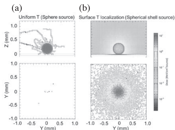
Fig. 3 Distribution of energy deposition from tritium (a) with uniform concentration through the tungsten dust and (b) localized in a shell of the tungsten dust to TIPT and the surrounding air.
