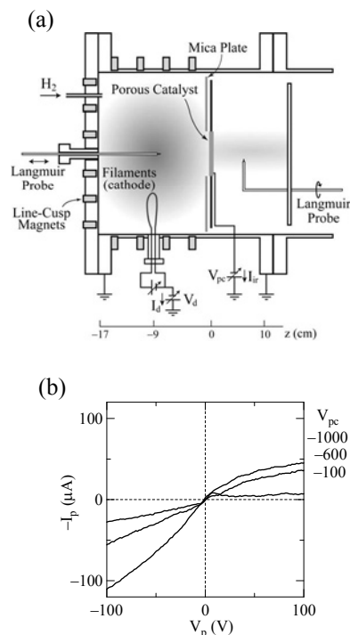
Fig. 1. (a) Experimental setup. Hydrogen plasma is generated by dc arc discharge and irradiated to porous nickel catalyst. Hydrogen atomic ions are produced from the back side of the irradiation plane. (b) I-V characteristics of Langmuir probe at z = 3 cm.
