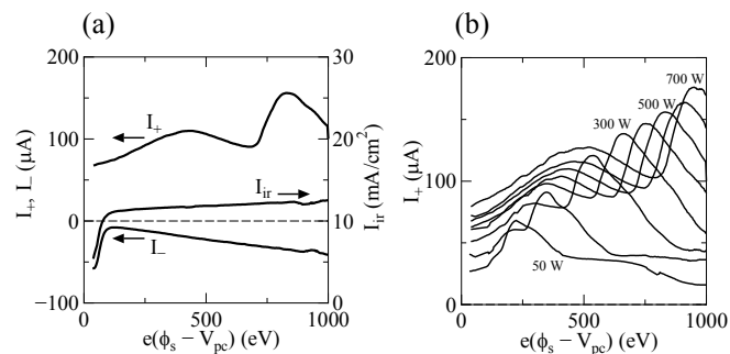
Fig. 2. (a) Probe saturation currents of positive and negative ions and the irradiation current as functions of the irradiation energy. (b) Dependence of peak energies appearing in positive-ion production on the discharge power.
