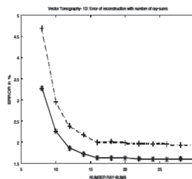
Fig. 2 Errors of reconstructed values as a function of projection number when 10% white noise is applied to the measured projection signals (+ : type 1 flow. ●: type 2 flow).
