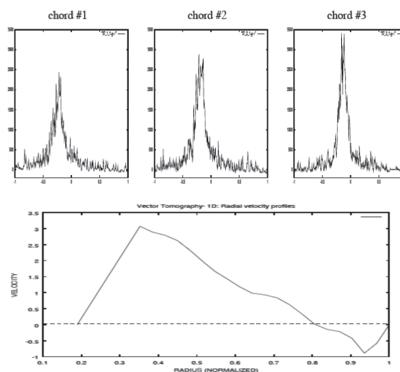
Fig. 3 Examples of HeII spectrums measured by 2-D Doppler diagnostics (top) and the radial velocity profile reconstructed from those data (bottom).
