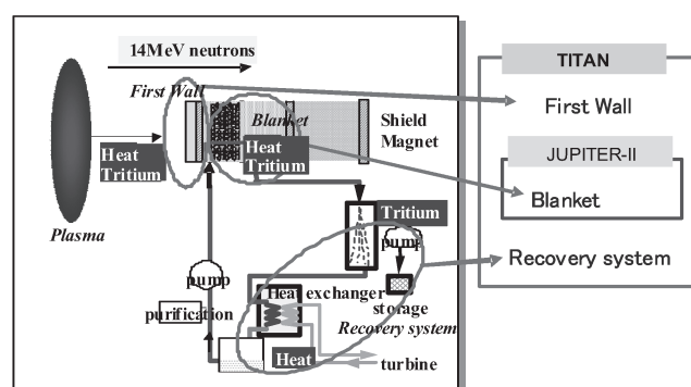
Fig. 1 Schematic illustration of the energy and tritium extraction system of fusion reactors. Also shown are the component system JUPITER-II and TITAN Projects cover.
