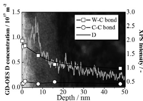
Fig Depth distributions of deuterium in \text{D}_2^+ fluence of 0.3 \times 10^{22}\text{ D}_2^+ \text{ m}^{-2} and chemical states of C in \text{C}^+ - \text{D}_2^+ sequential implantation, and TEM image in 5.0 \times 10^{21}\text{ C}^+ \text{ m}^{-2}
