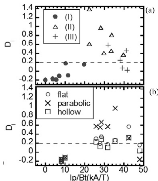
Fig. 2. Temporal evolution of Mercier parameter D_I until minor collapse. (a) B_t = -1.266 T, (b) B_t = -0.75 T.
