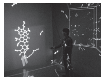
Fig. 2. CAVE visualization of molecular dynamics simulation results.
