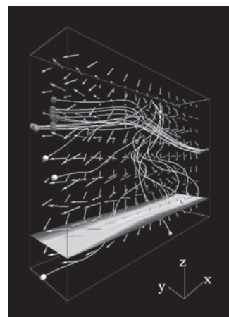
Fig. 1. CAVE visualization of plasma particle simulation results.
