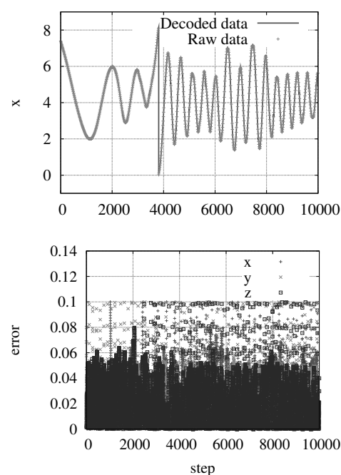
Fig. 1. Reproducibility and error between the simulation and the decoded data. (top) Time evolution of the particle x coordinates is shown. Red line indicates the decoded data, and green plus symbol shows the simulation data. (bottom) Errors (difference) between the simulation and decoded data are shown. Plus, cross and square symbols are the errors for x , y and z coordinates, respectively.
