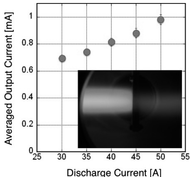
Fig. 3: Averaged output current as a function of the discharge current. The inset of the figure is the photograph showing the TEC module irradiated by a high density He plasma in the NAGDIS-II device.
