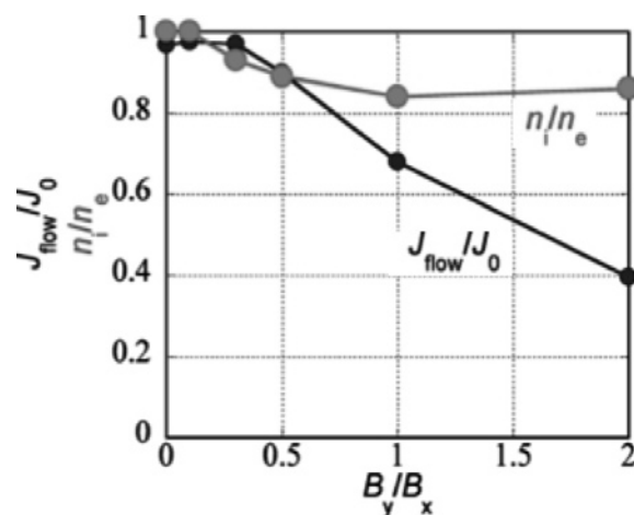
Fig. 2: Simulation result of the output current as a function of the magnetic field strength B_y . B_x is 0.1 T.
