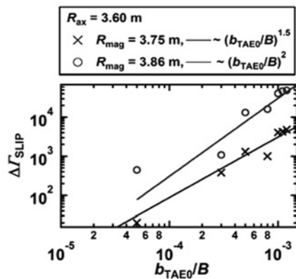
Fig. 2 Fast-ion loss due to TAE \Delta\Gamma_{SLIP} dependence on fluctuation amplitude at TAE peak b_{TAE0}/B in calculation.
