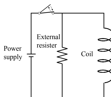
Fig. 2. Quench protection circuit.
