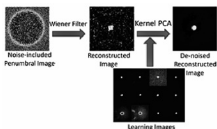
Fig. 1. Basic concept of the removal of the artifact in the reconstructed image by the use of the kernel principal component analysis.
