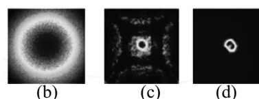
Fig. 3. Experimental setup for real laser-plasma experiments(a), obtained penumbra image(b), reconstructed image by the conventional method (c), and reconstructed image by the proposed method(d)
