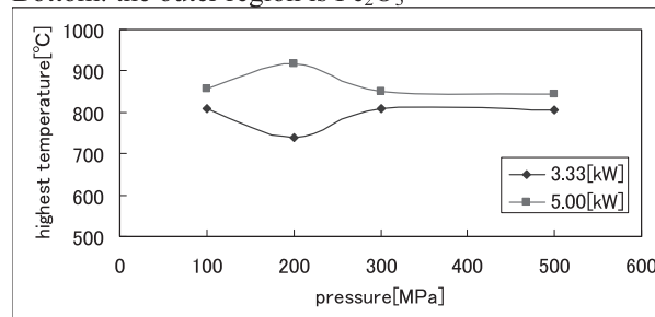
Fig. 3 Maximum temperature dependence on the pressure of the green compact
