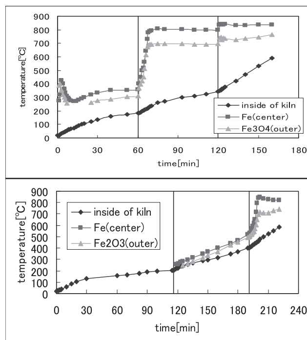
Fig.2 Temperature of the sample during microwave sintering.
