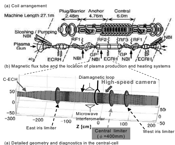
Fig.1 Schematic of GAMMA 10 and camera location
