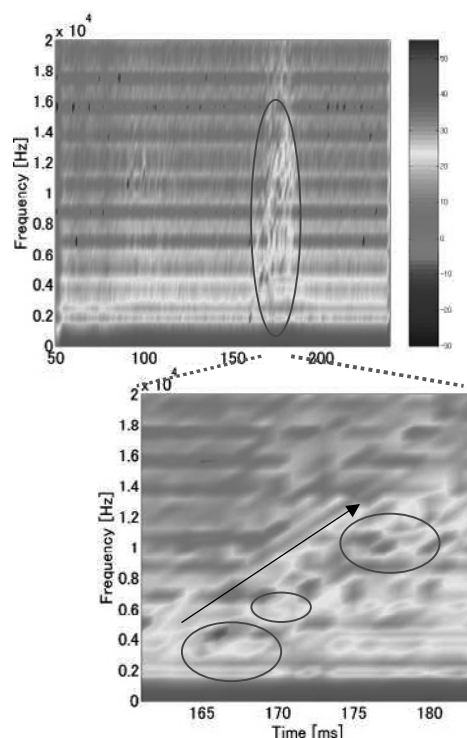
Fig.3 Power spectra of camera image Time-dependent FFT was applied to the data of specific pixel in the white circle shown in Fig.2
